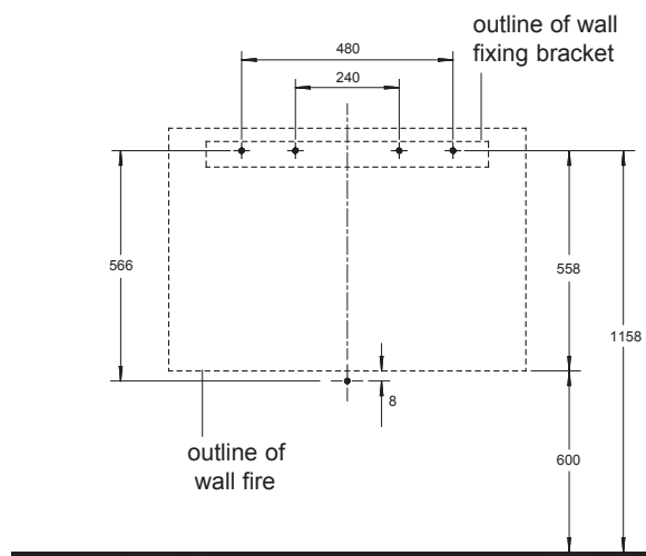
Recommended Fixing Dimensions - Fig. 2
