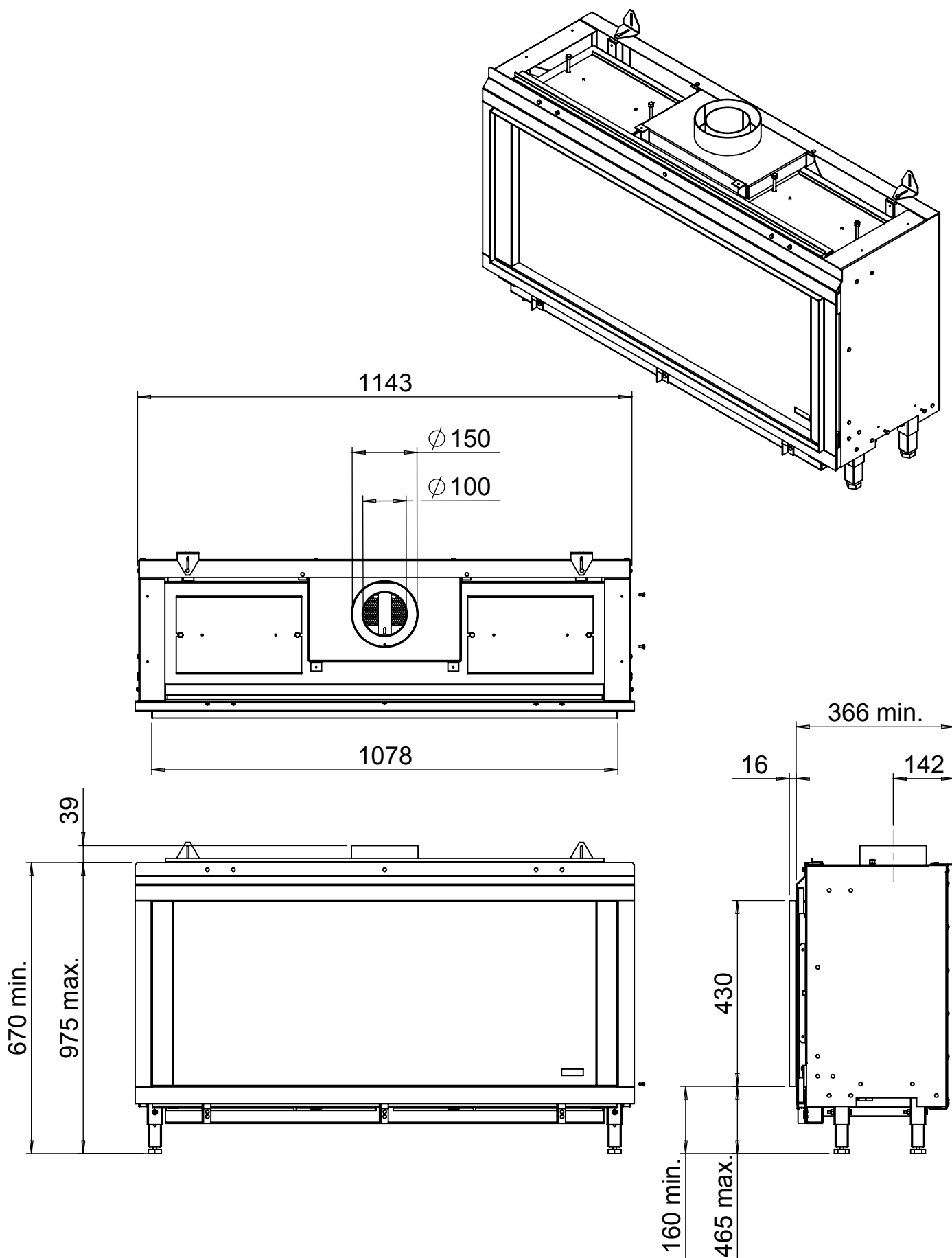
Dimensional drawing Relaxed L Smart
